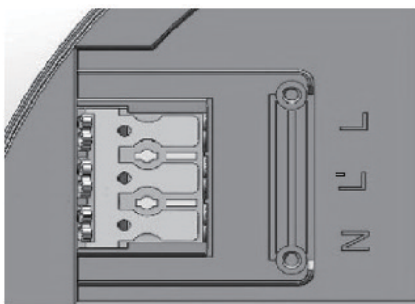
Terminal of luminaire with motion sensor
