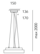
Wire suspension 300/400
