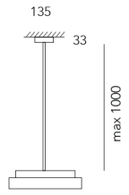
Rod suspension
