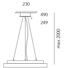
Wire suspension 600
