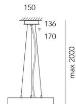
Central wire suspension 320/450
