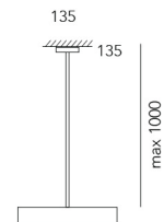
Rod suspension
