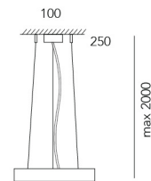
Parallel wire suspension
