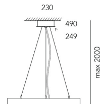
Central wire suspension 600/900
