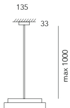
Rod suspension
