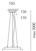
Wire suspension 300/400
