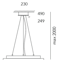
Wire suspension 600
