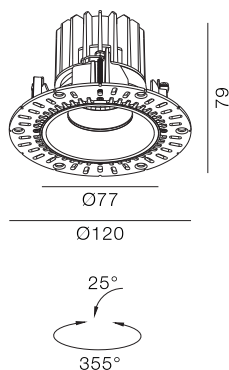
Classic Trimless Tilt IP44
