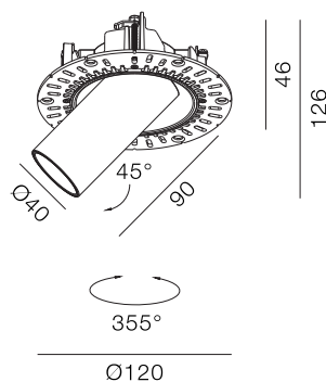
Classic Trimless Spot IP20
