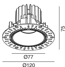
Classic Trimless Fix IP44
